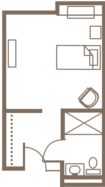
STUDIO 300 sq. ft.
