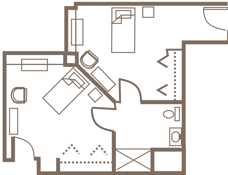
SHARED SUITE 510 sq. ft.
